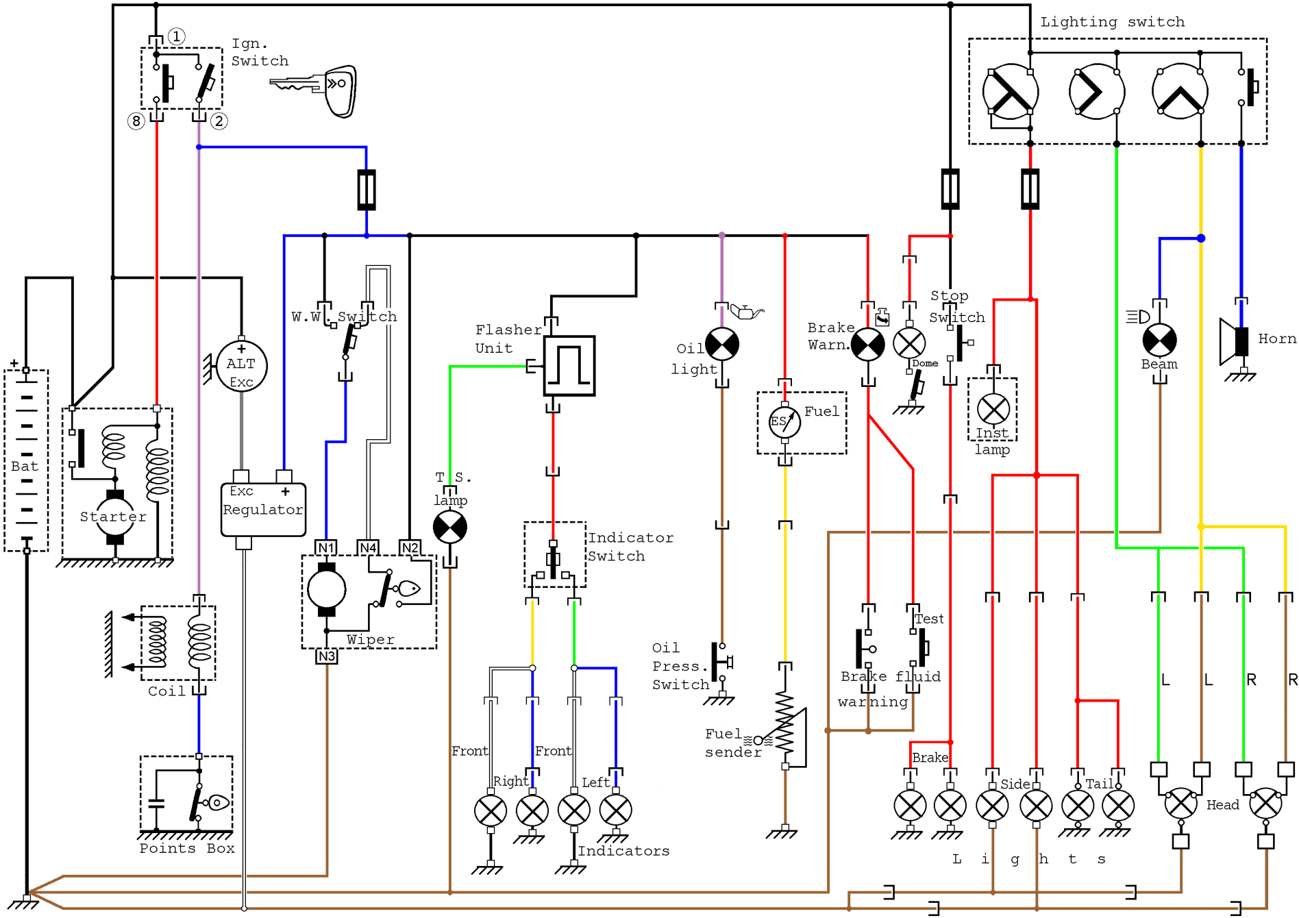
Wiring diagram - 2CV 1981
